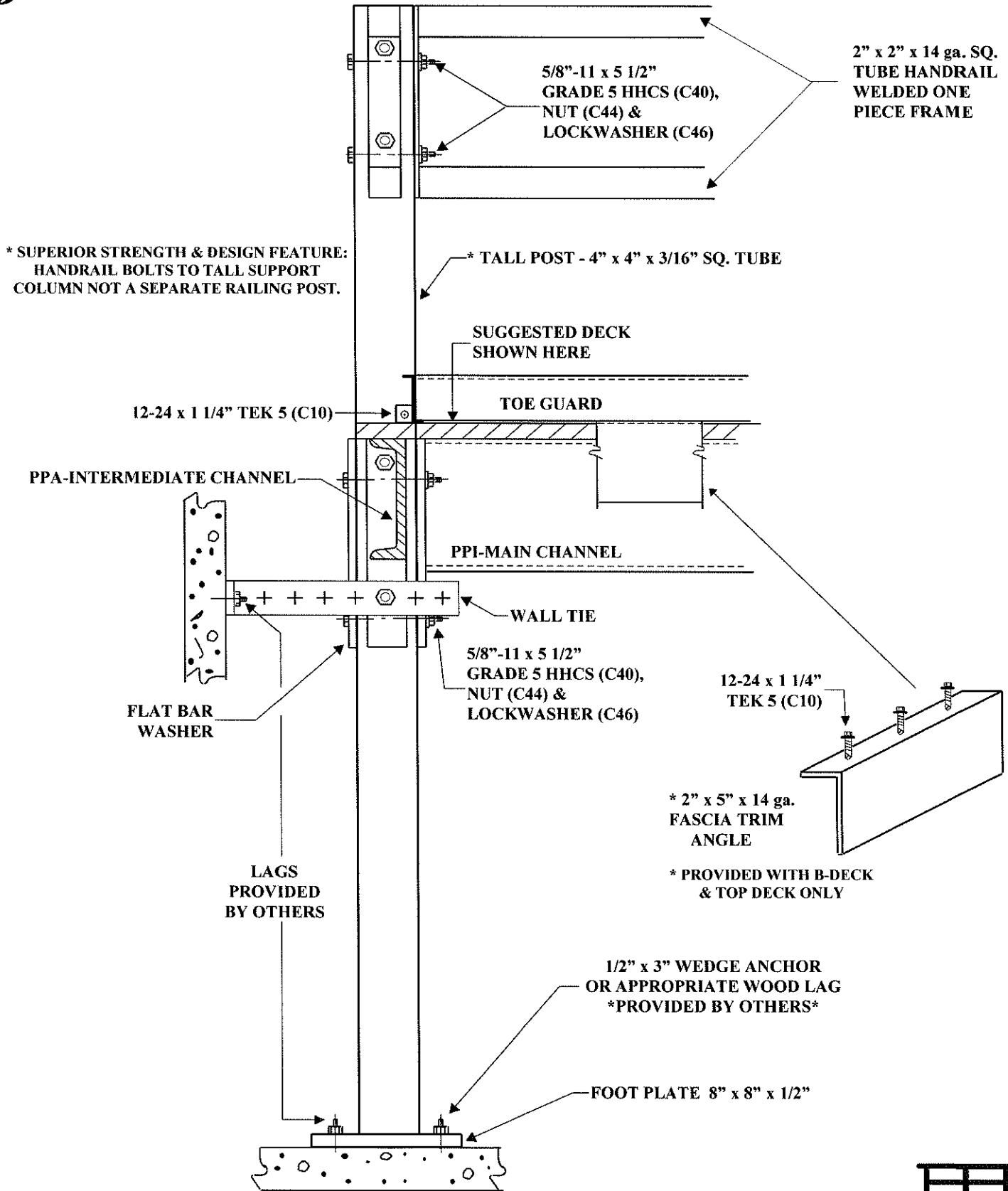
TYPICAL SIDE VIEW THROUGH PPA CHANNEL
