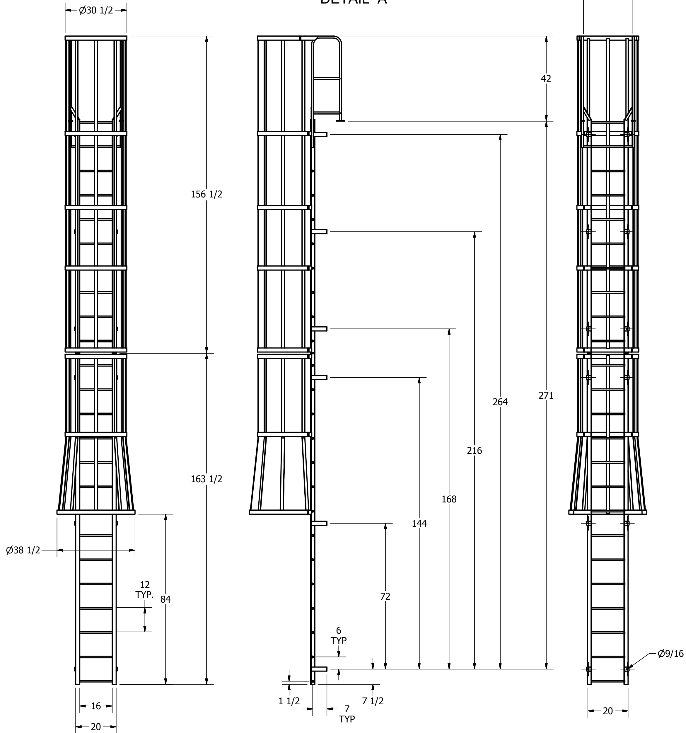
DETAIL A
