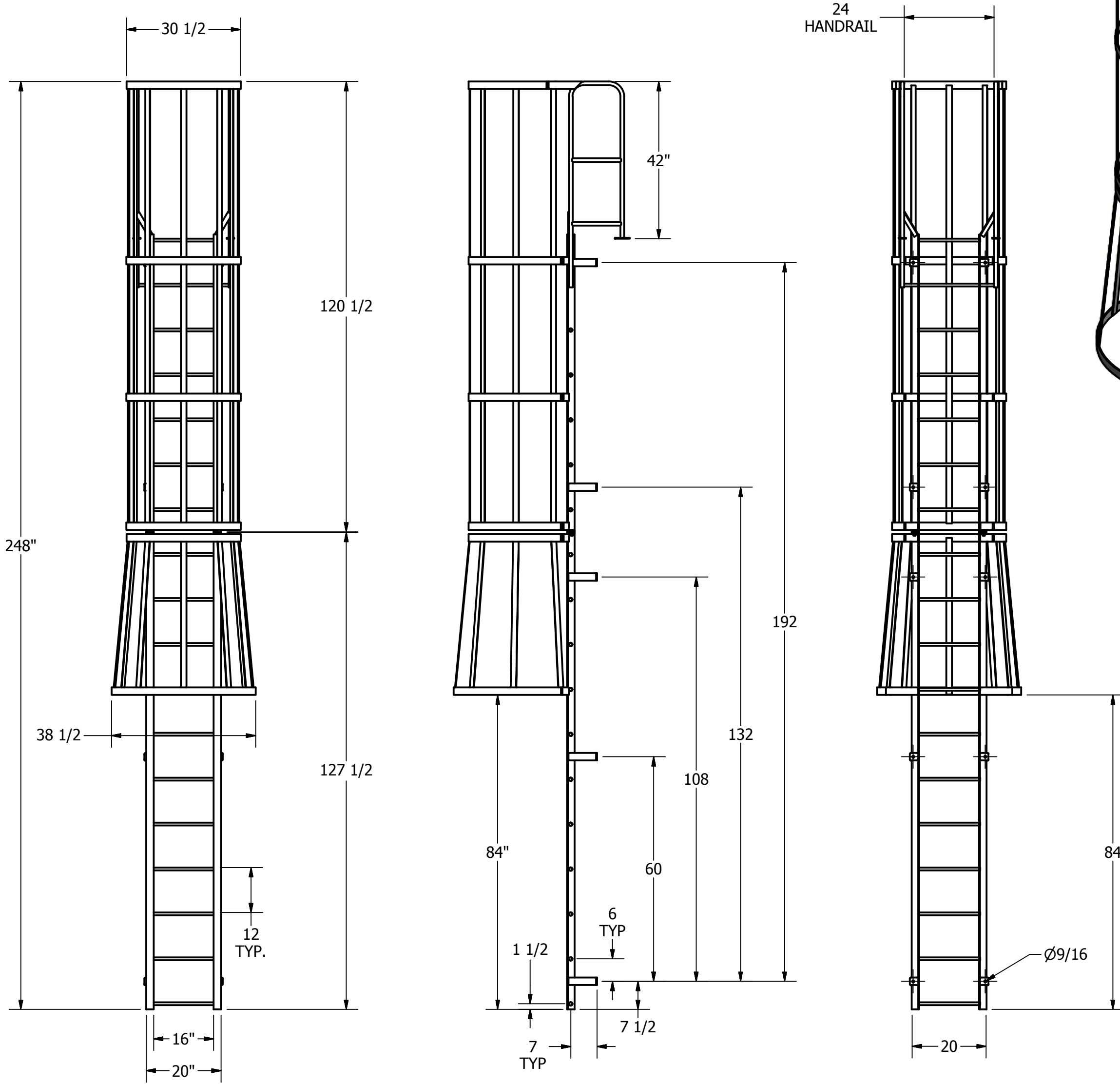
DETAIL A
