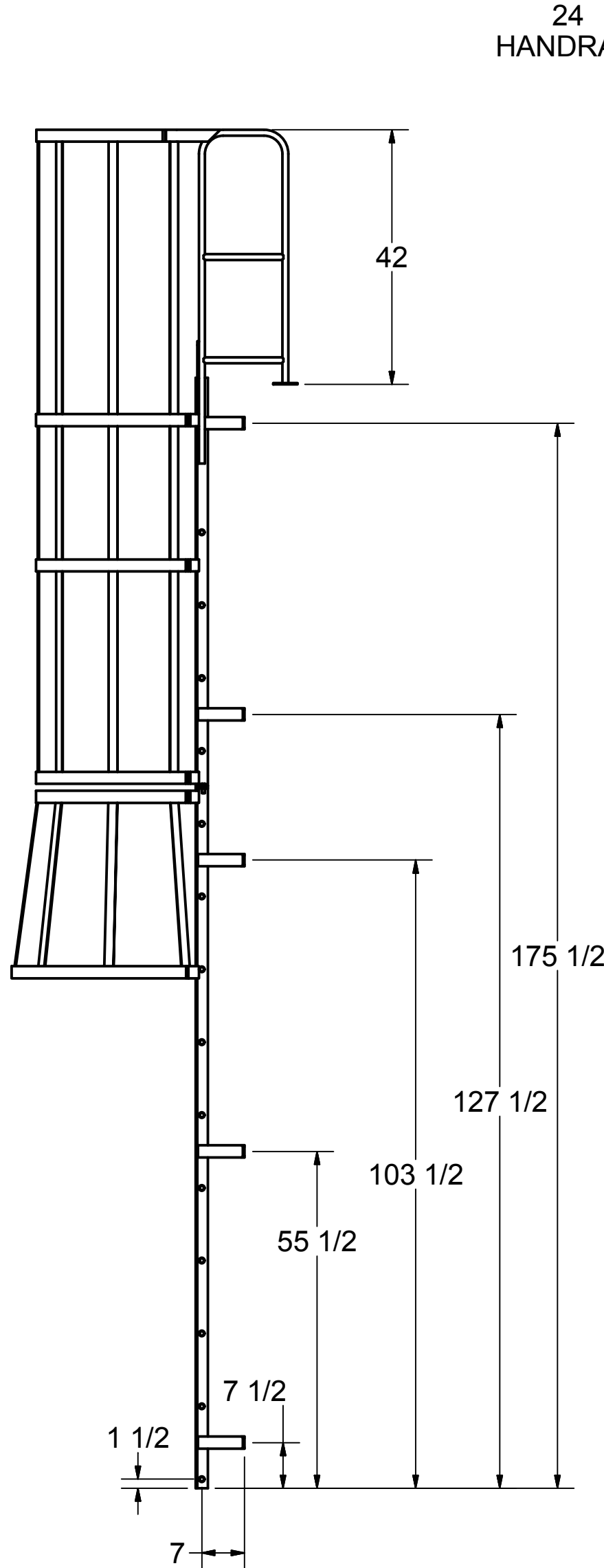
DETAIL A
