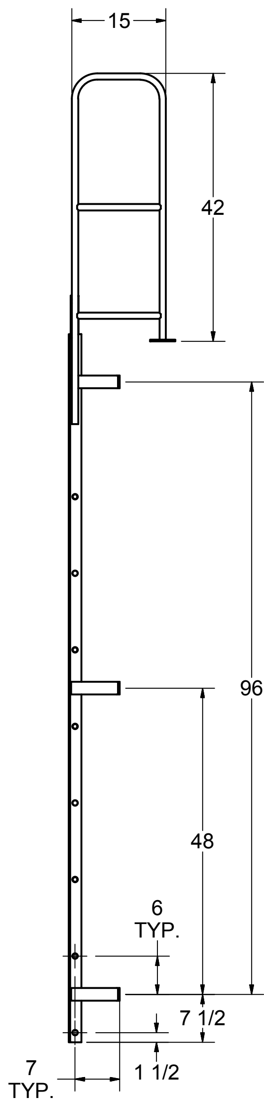
DETAIL A
